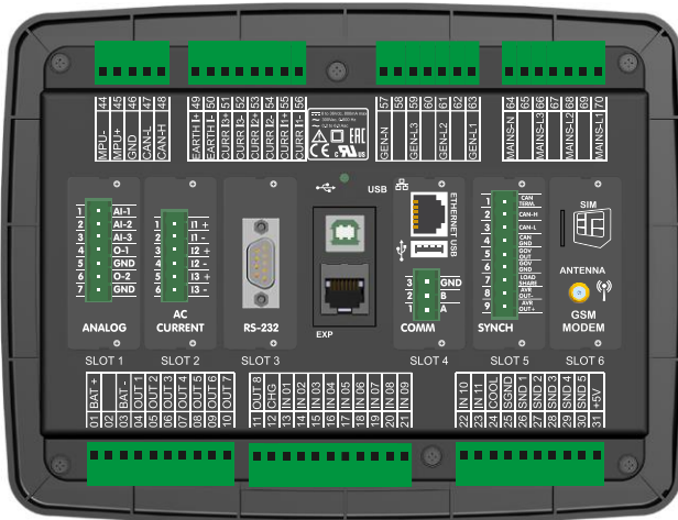
Backpanel view
